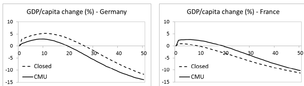
Figure 1. Simulation results, population ageing, no social security reform
